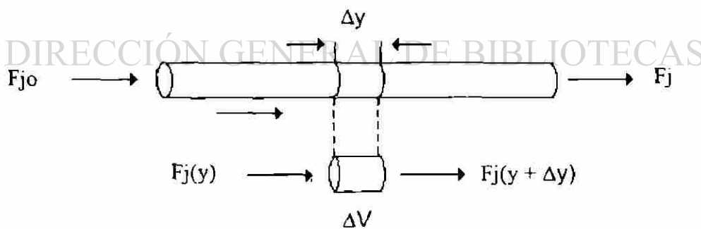
Figura 7. Reactor tubular
