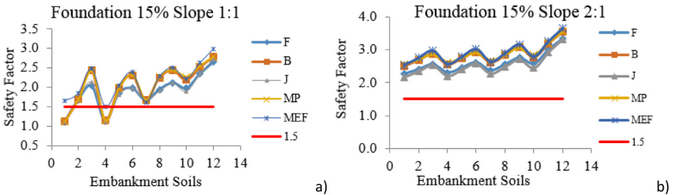
Fig. 7. Safety-factor graphs taking into account the methods and soils used for embankments, 6 m high with 15% of CBR in the foundation (a) with slope 1:1 and, (b) with slope 2:1.
