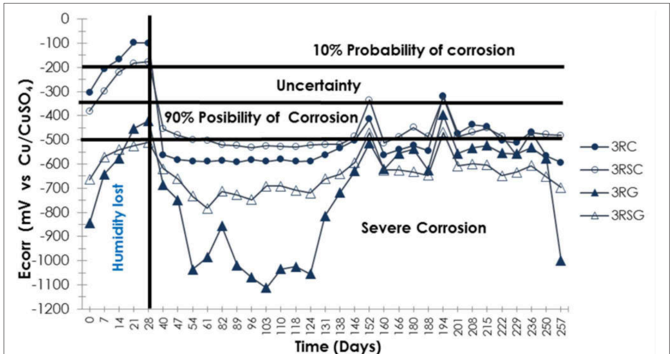
FIGURE 6 | E_{corr} specimens in soil type MH with 3% of NaCl.
