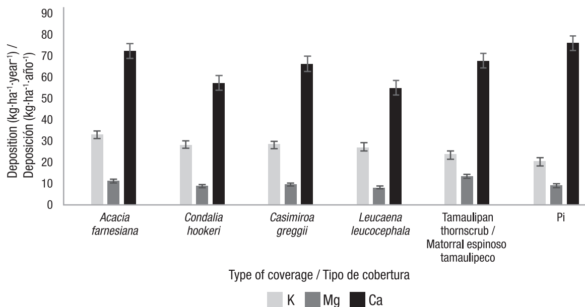
Figure 2. Contribution of macronutrients via throughfall for each plant canopy and via gross rainfall (Pi).
