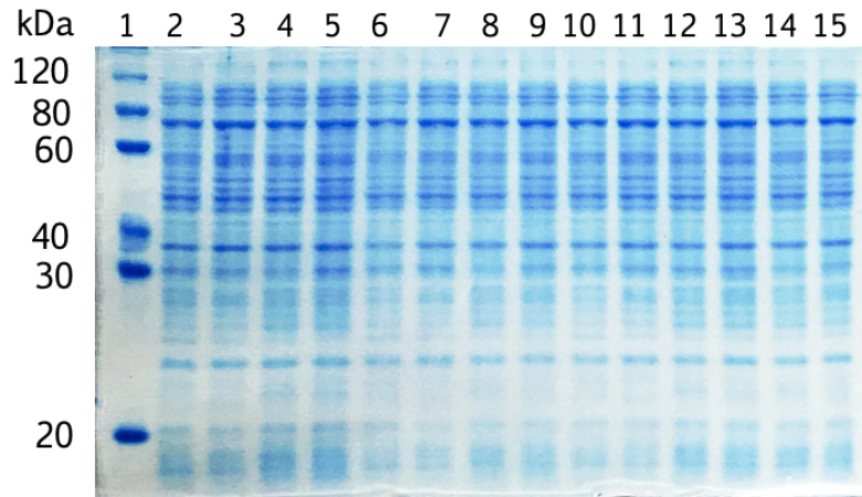
Figura 33. Análisis de fracciones del tratamiento por congelación/descongelación y detergentes iónicos a 4°C. Carril 1: marcador de peso molecular, carril 2: 0.1% CHAPS 1hora, carril 3: 0.1% CHAPS 24 horas, carril 4: 0.3% sarcosil 1 hora, carril 5: 0.3% sarcosil 24 horas, carril 6: 1 mM BME 1 hora, carril 7: 1mM BME 24 horas, carril 8: 0.1% CHAPS + 0.3% sarcosil 1hora, carril 9: 0.1% CHAPS + 0.3% sarcosil 24 horas, carril 10: 0.1% CHAPS + 1 mM BME 1 hora, carril 11: 0.1% CHAPS + 1 mM BME 24 horas, carril 12: 0.3% sarcosil + 1 mM BME 1 hora, carril 13: 0.3 sarcosil + 1 mM BME 24 horas, carril 14: 0.1% CHAPS + 0.3% sarcosil + 1 mM BME 1 hora, carril 15: 0.1% CHAPS + 0.3% sarcosil + 1 mM BME 24 horas.
