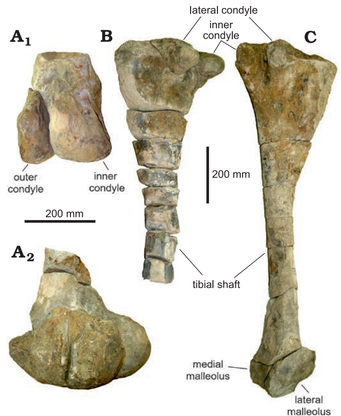
Fig. 5. Hindlimb elements of Lambeosaurinae indet. (FCBUANL_2711) from Ejido Presa San Antonio, Coahuila, Mexico, upper Campanian. A. Distal end of the left femur, in caudal (A 1 ) and lateral (A 2 ) views. B. Left tibia in lateral view. C. Right tibia in lateral view.
