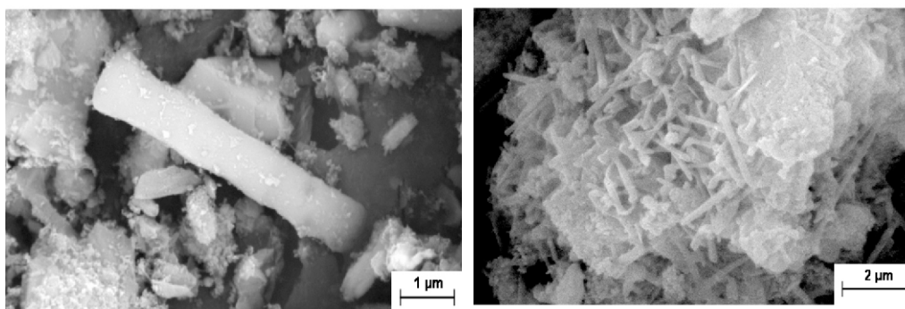
Figure 8. a) SEM micrograph in backscattered electron mode of rice hulls after pyrolysis for six hours at 1250°C in a nitrogen atmosphere, b) SEM micrograph in backscattered electron mode of an agglomerate obtained from ashes after pyrolysis for six hours at 1400°C in nitrogen.
