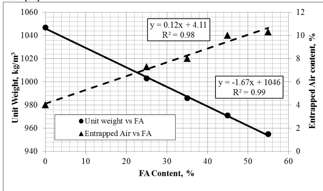
Figure 4. Effect of FA substitutions on unit weight and air content of fresh mortars with w/b 1 (0.6).
