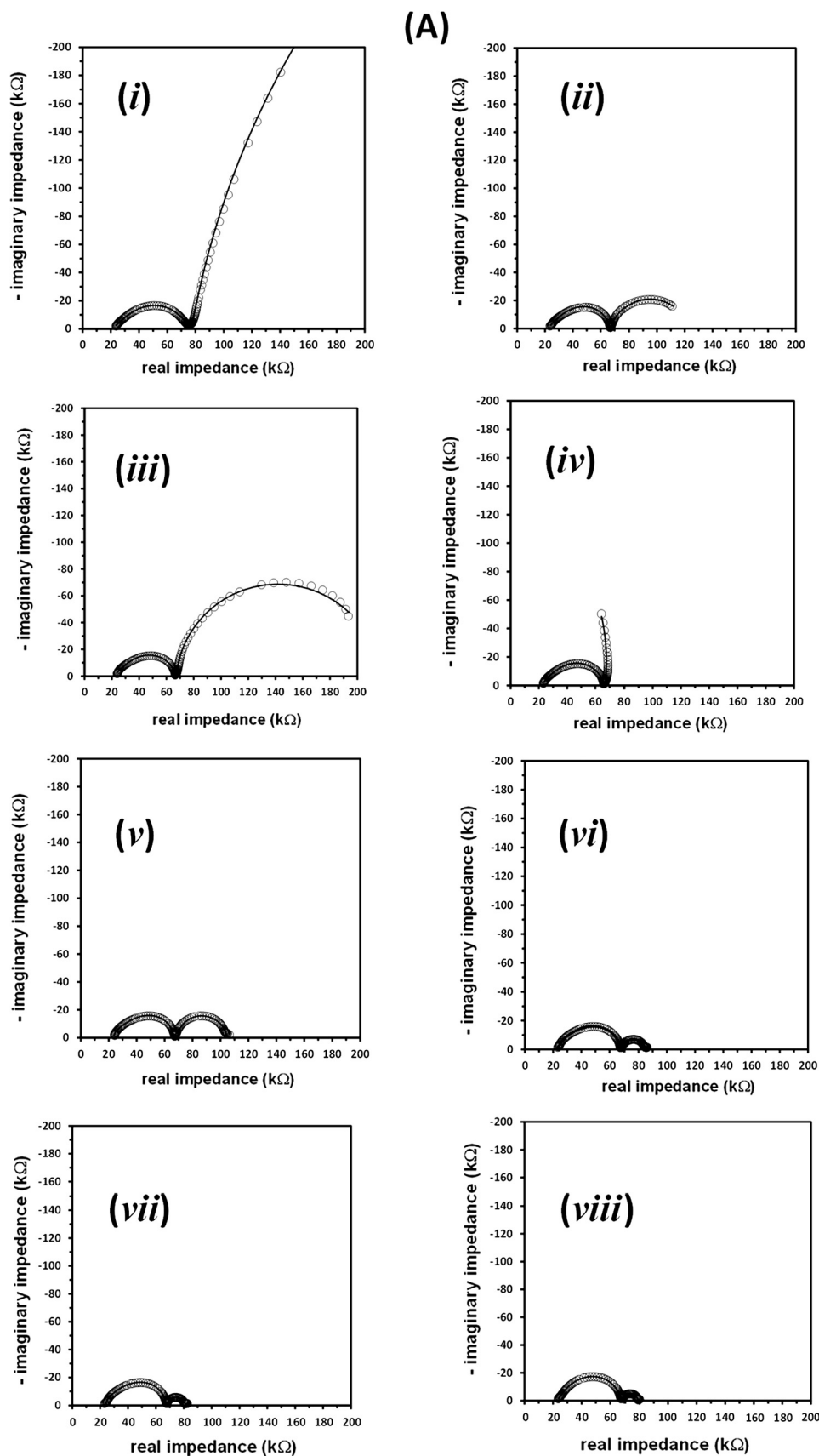
Fig. 8 (A) Circles are the experimental EIS spectra obtained for polarized \text{TiO}_2 -bearing anodes (ITO/ \text{TiO}_2 // \text{Ni}^{\text{II}} cyclam) at 0.4 (i), 0.5 (ii), 0.6 (iii), 0.7 (iv), 0.8 (v), 0.9 (vi), 1.0 (vii) and 1.1 V (viii) vs. RE1, immersed in a deoxygenated solution of aqueous 0.1 M NaOH plus 10 mM urea at 25 °C. Solid lines corresponds to the best fitting of the equivalent circuit displayed in (B) to the experimental spectra.
