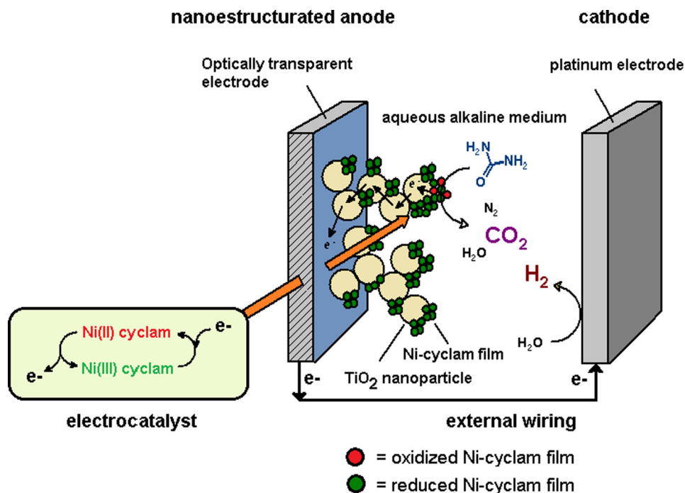
Scheme 1 Representation of the electrochemical cell proposed to conduct studies on urea electrolysis (anode, via Eq. (11)) and simultaneous \text{H}_2 generation (cathode, via Eq. (12)).
