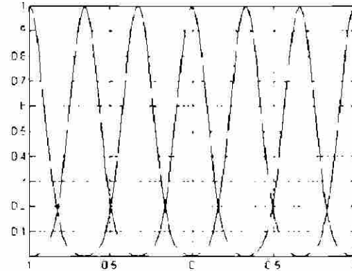
Fig. 1 - Gaussians Fuzzy Sets
