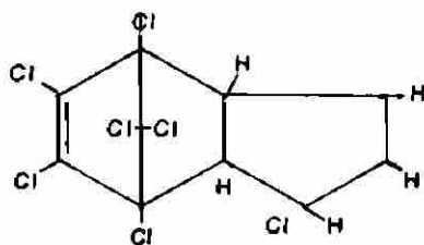
1,4,5,6,7,8,8-HEPTACLORO-3 \alpha ,4,7,7 \alpha -TETRAHIDRO-4,7-METANO-1H-INDENO
