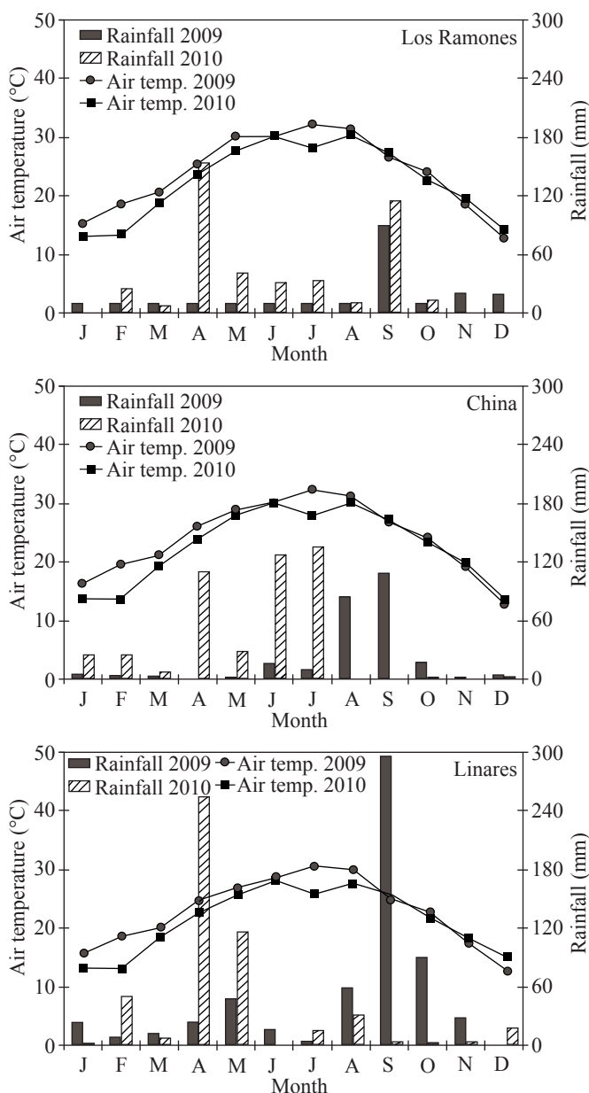
Figure 1: Monthly mean air temperature and monthly rainfall during 2009 and 2010 at Los Ramones, China and Linares, north-eastern Mexico
