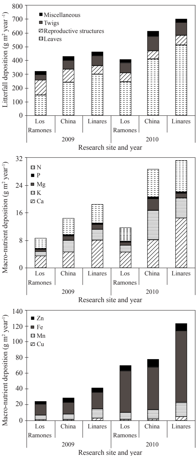
Figure 2: Litterfall, macro- and micro-nutrient deposition during 2009 and 2010 at research sites, north-eastern Mexico
